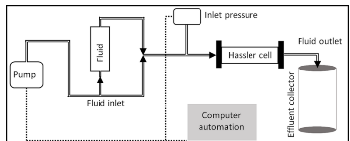
Figure 1: Experimental core flooding testing set up
